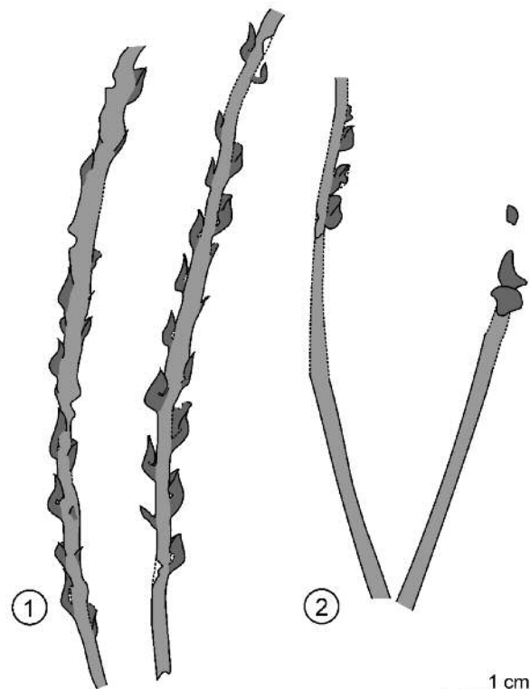
Type 3c: Zosterophyllum from Newton Dingle
