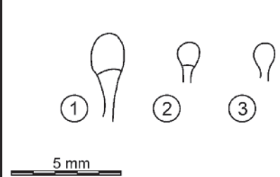
Type 1e: "Zosterophylloid" sporangia
