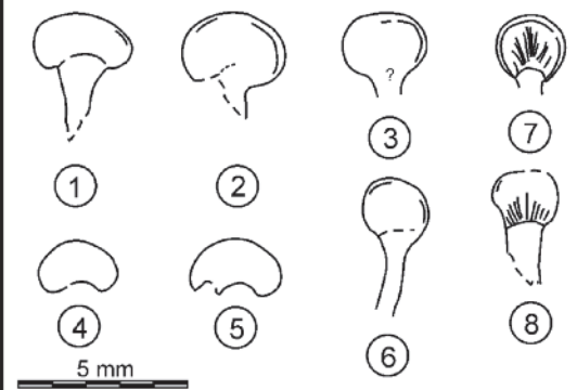
Type 1e: "Zosterophylloid" sporangia
