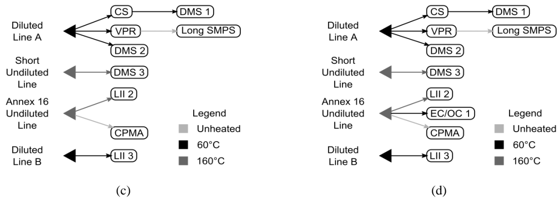
Fig. 2 Aerosol instrumentation used for: (a) CFM56-5B4/2P turbine engine on April 29 th 2012; (b) CFM56-5B4/2P turbine engine on April 30 th 2012; (c) CFM56-7B26/3 turbine engine on May 2 rd 2012; (d) PW4000-100 turbine engine on May 3 rd 2012. The arrangement of the CPMA-mDMS relative to the AMS system (Fig. 2b) is shown in Fig. 3.
