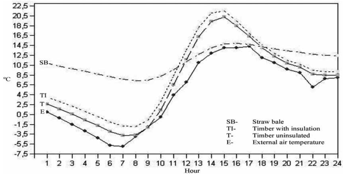
Fig. 3. Dry Bulb Temperatures 31 st July (winter) simulated with TAS software
