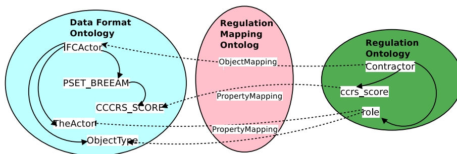
Figure 7: Data Mapping
