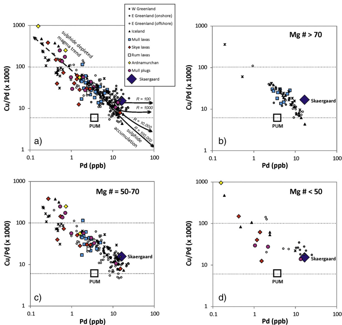
Fig. 10. PGE ratio plots. Cu/Pd vs. Pd according to Mg#; (a) all lavas, (b) lavas with Mg# > 70, (c) lavas with Mg# 50–70, (d) lavas with Mg# < 50. Primitive mantle from McDonough and Sun (1995). Sulphide depletion vector calculated from silicate/sulphide partition coefficients (Mungall and Brenan, 2014) for R factors (silicate/sulphide ratio) of 100 to 100,000. Skaergaard chilled composition (blue diamond) based on 265 ppm Cu (calculated by Thomassen and Nielsen, 2006) and 17 ppb Pd (chilled margin analysis by Vincent and Smales, 1956).
