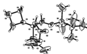
Figure 3 The structure of the oxazolidinone 5 as established by X-ray diffraction.
