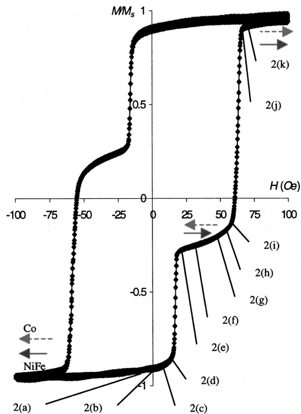
FIG. 3. Normalized magnetization vs applied field for the NiFe/Al-oxide/Co junction film. The corresponding domain structure at different field values along the hysteresis loop is shown in Fig. 2.
