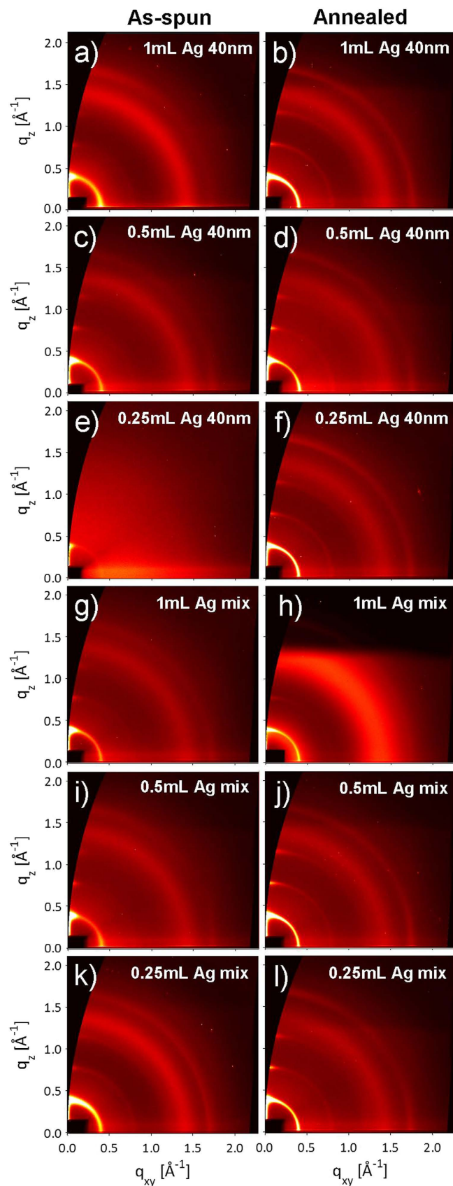
Figure 5. Diffraction images collected at the critical angle for as-spun and annealed P3HT: PCBM: Ag NPs blends: (a-b) Ag 40 nm 1 mL, (c-d) Ag 40 nm 0.5 mL, (e-f) Ag 40 nm 0.25 mL, (g-h) Ag mix 1 mL, (i-j) Ag mix 0.5 mL, and (k-l) Ag mix 0.25 mL. Images are extracted at the critical angle in order to display the maximum intensity.
