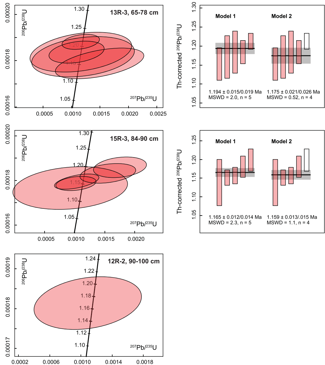
Figure 4. U-Pb concordia diagrams and weighted mean ^{206}\text{Pb}/^{238}\text{U} plots of single-grain and grain fragment zircon dates. All data are corrected for initial ^{230}\text{Th} exclusion as described in the text. Ages on concordia are in Ma. Plots and weighted mean calculations were generated using the U-Pb_redux software package [Bowring et al. , 2011; McLean et al. , 2011]. The weighted mean plots include the weighted mean of the entire data set (model 1) and the weighted mean excluding the oldest date (model 2). Data from fractions 15-3 z3 and 12-8A z3-2 are excluded from the plots for clarity.
