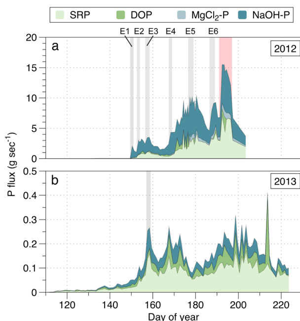
Figure 5. Time series of calculated phosphorus fluxes at (a) Leverett Glacier and (b) Kiattuut Sermia. Only “bioavailable” phosphorus fractions are shown (dissolved P phases plus MgCl_2\text{-P} and NaOH\text{-P} ). Dissolved fluxes are represented with green colors, and particulates fluxes with blue/grey colors. Fluxes are cumulative at each time point. Grey shaded areas in Figure 5a are indicative of outburst events (E) and in Figure 5b of a significant hydrological shift in the glacial drainage system (a spring event). The red shaded area in Figure 5a highlights the 2012 record melt event.
