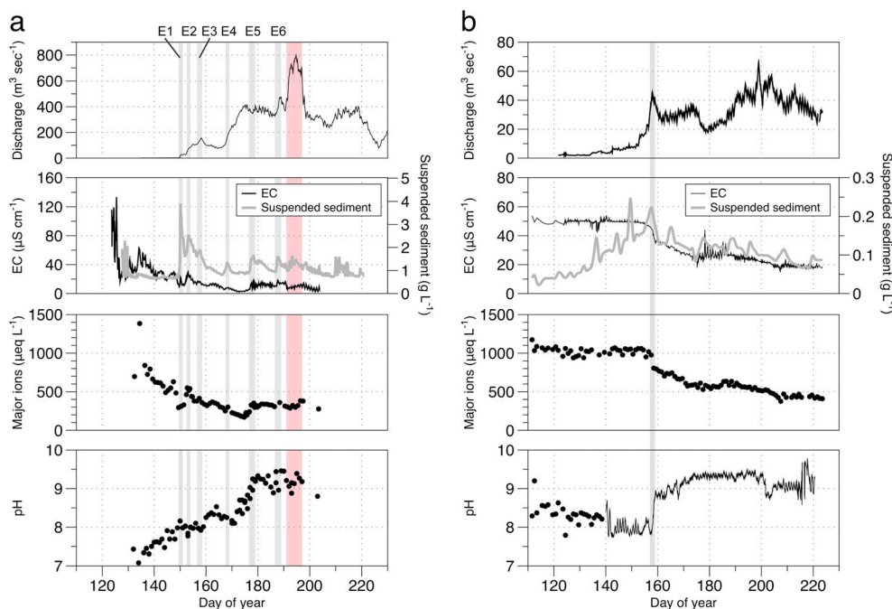
Figure 2. Hydrological and geochemical data for (a) Leverett Glacier and (b) Kiattuat Sermiat. Grey shaded areas in Figure 2a are indicative of outburst events (E) and in Figure 2b of a significant hydrological shift in the glacial drainage system (a “spring event”). The red shaded area in Figure 2a highlights the 2012 record melt event.
