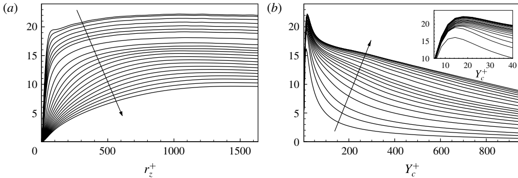
FIGURE 2. Behaviour of scale energy in the r_y = 0 plane. (a) Plot of \langle \delta u^2 \rangle as a function of r_z for different wall distances from its maximum at Y_c^+ = 18 to Y_c^+ = 900 . The arrow indicates increasing wall distances. (b) Plot of \langle \delta u^2 \rangle as a function of Y_c for different r_z . The arrow indicates increasing spanwise separations. The inset plot is an enlargement of the near-wall behaviour.
