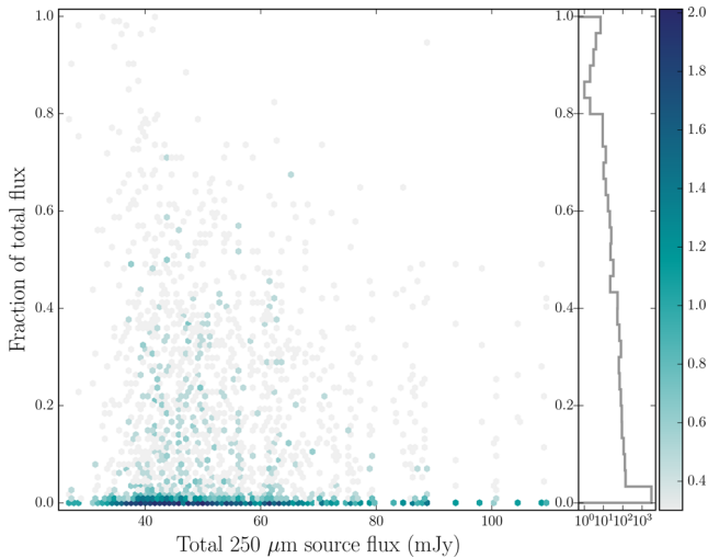
Figure 3. Left-hand panel: the unbinned data points for all potential components in our sample, plotted as a density histogram. We plot the fraction of the total 250- \mu\text{m} source flux assigned to each potential component, as a function of the total 250- \mu\text{m} flux. Colour indicates the log of the number of points contained within that bin, as indicated by the colour bar on the far right. Points close to 1 on the y-axis indicate that they were assigned almost 100 per cent of the total flux, meaning that they are the only source assigned significant flux. For high total flux 250- \mu\text{m} sources, there is a deficit of components at large flux fractions (i.e. high-flux objects tend to have that flux divided amongst more components, explored in more detail in text). The right-hand panel shows a histogram of the distribution of flux fractions across all 250- \mu\text{m} source fluxes. The x-axis in the right-hand panel is in log space.
