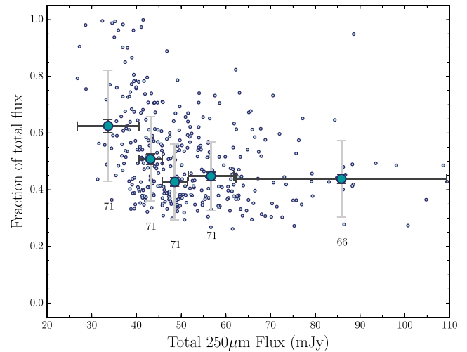
Figure 4. For each 250- \mu\text{m} source, we select the component with the highest assigned flux fraction. We plot these brightest components as a function of the total 250- \mu\text{m} flux in small background points. Horizontal error bars on the larger, binned points indicate the width of the bin, and the numbers below each point indicate the number of brightest components within each bin. Pale vertical error bars show the standard deviation on the distribution of all possible medians, including both the flux uncertainty and the dispersion of brightest component contained within the bin. Black vertical error bars (typically of comparable size to the data point) are calculated by dividing the pale error bars by \sqrt{n} , applicable as each data point is an independent measurement and measurement error should not introduce a systematic bias. We refer to the black \sqrt{n} error bars for the remainder of this work. The brightest components show a trend towards higher fractions of 250- \mu\text{m} flux as total 250- \mu\text{m} flux decreases. A Spearman Rank correlation test on the unbinned data gives a p -value of 1.86 \times 10^{-12} , which excludes the null hypothesis of no correlation at >6\sigma .
