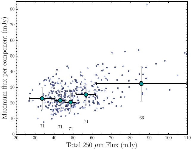
Figure 5. The same as Fig. 4, but now plotting the flux value assigned to the brightest component instead of the fraction of the total flux. The brightest components at high 250- \mu\text{m} fluxes are still brighter than the low 250- \mu\text{m} flux components. A Spearman Rank correlation test on the unbinned data gives a p -value of 1.08 \times 10^{-13} , indicating an exclusion of the null hypothesis of no correlation at >7\sigma .
