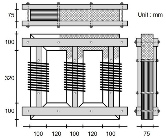
a) Three phase core
