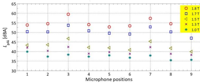
Fig. 8. Variation of averaged (3 trials) A-weighted sound pressure level from microphone placed on the prescribed contour (positions 1 to 8) and above (position 9) of three phase MSL CGO core at flux densities of 1.0 T to 1.8 T, 50 Hz.
