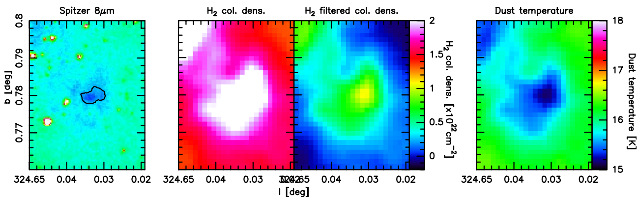
Fig. 1: Images of SDC324.633+0.779. From left to right: Spitzer 8\mu\text{m} image with the \tau_{8\mu\text{m}} = 0.35 opacity contour showing the boundary of the SDC as defined in PF09; Herschel \text{H}_2 column density map with background; Herschel background filtered \text{H}_2 column density map; Herschel dust temperature map.
