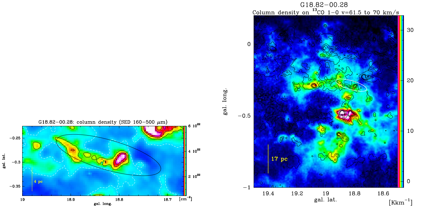
Fig. A.4. Left: column density map of G18.82-0.28, obtained from SED-fit to Herschel 160, 250, 350, 500 \mu\text{m} data. Black contours indicate the levels N_{dust}=2 to 5 \times 10^{22} \text{ cm}^{-2} in steps of 10^{22} \text{ cm}^{-2} , white-dashed contour outlines the approximate completeness level, and ellipse is taken from Simon et al. (2006b), defining the IRDC. Right: line integrated ^{13}\text{CO} 1 \rightarrow 0 emission in colour scale (in [\text{K km/s}] between v=61 and 70 \text{ km s}^{-1} , the velocity range of the bulk emission of G18.82-0.28 and the associated GMC. Note that this GMC was already identified as a coherent cloud complex in Schuller et al. 2009. The Herschel \text{H}_2 column density is overlaid as black contours (levels 1,2,3,4,5 10^{22} \text{ cm}^{-2} ) and the IRDC is outlined by an ellipse (Simon et al. 2006b).
