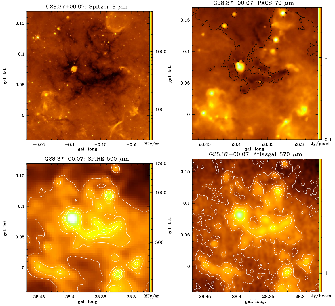
Fig. 1. Top: Spitzer 8 \mu\text{m} ( \sim 2.5'' resolution) and PACS 70 \mu\text{m} maps ( \sim 11'' resolution). The Spitzer / IRAC data were taken from the public available GLIMPSE archive. Bottom: SPIRE 500 \mu\text{m} map ( 36'' resolution) and ATLASGAL 870 \mu\text{m} maps ( 23'' resolution) of G28.37+0.07. The central dark feature in the Spitzer and PACS images is the IRDC, appearing bright at longer wavelengths (SPIRE and ATLASGAL).
