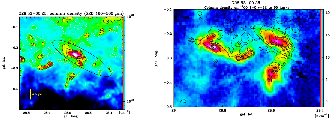
Fig. A.6. Left: column density map of G28.53-0.25, obtained from SED fit to Herschel 160, 250, 350, 500 \mu\text{m} data. Black contours indicate the levels N_{\text{dust}}=2.5, 3, 4, 6 \times 10^{22} \text{ cm}^{-2} , white-dashed contour outlines the approximate completeness level, and ellipse is taken from Simon et al. (2006b), defining the IRDC. Right: line integrated ^{13}\text{CO} 1 \rightarrow 0 emission (in [K km/s]) between v=82 and 90 \text{ km s}^{-1} , the velocity range of the bulk emission of G28.53-0.25, and the associated GMC. The Herschel \text{H}_2 column density is overlaid as black contours (levels 2, 2.5, 3, 4, 6 10^{22} \text{ cm}^{-2} ) and the IRDC is outlined by an ellipse (Simon et al. 2006b).
