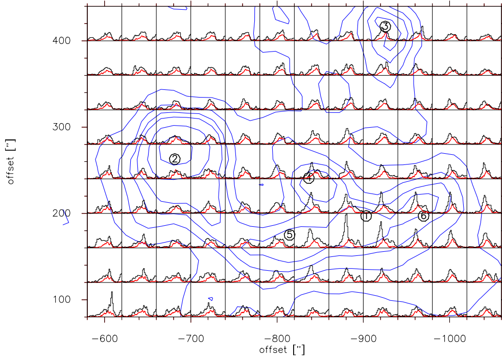
Fig. 9. Main beam brightness temperature spectra of ^{12}\text{CO} 3 \rightarrow 2 (black) and ^{13}\text{CO} 1 \rightarrow 0 (red) emission in the velocity range 55 to 95 \text{km s}^{-1} and temperature range -0.2 to 12 K. The area corresponds to the centre region of the IRDC G28.37+0.07, outlined in Fig. 8. The dust column density from Herschel is overlaid as blue contours (levels 4, 5, 7, 10, 16 10^{22} \text{ cm}^{-2} ), and the numbering from 1 to 6 indicates the position of submm-continuum sources labelled using ATLASGAL and subsequently observed in \text{N}_2\text{H}^+ (Tackenberg et al. 2014).
