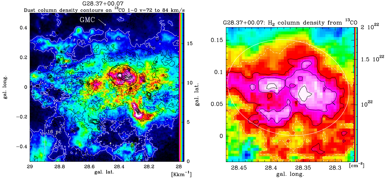
Fig. 3. Left: line integrated ^{13}\text{CO} 1\rightarrow 0 emission in colour scale between v=72 and 84\text{ km s}^{-1} , the velocity range of the bulk emission of the IRDC, and the associated GMC. The white contour indicates the 3.5\text{ K km s}^{-1} level, corresponding to A_v=2 , which defines the extent of the GMC and was used for mass estimation. The Herschel column density is overlaid as black contours (levels 2 to 6\times 10^{22}\text{ cm}^{-2} in steps of 10^{22}\text{ cm}^{-2} ) and the IRDC is outlined by an ellipse (Simon et al. 2006b). Right: \text{H}_2 -column density map of the centre region of the GMC, obtained from ^{13}\text{CO} 1\rightarrow 0 . The white-dashed contour indicates a column density of 1.25\times 10^{22}\text{ cm}^{-2} , the remaining black contours the levels 1.5 , 1.75 , and 2\times 10^{22}\text{ cm}^{-2} .
