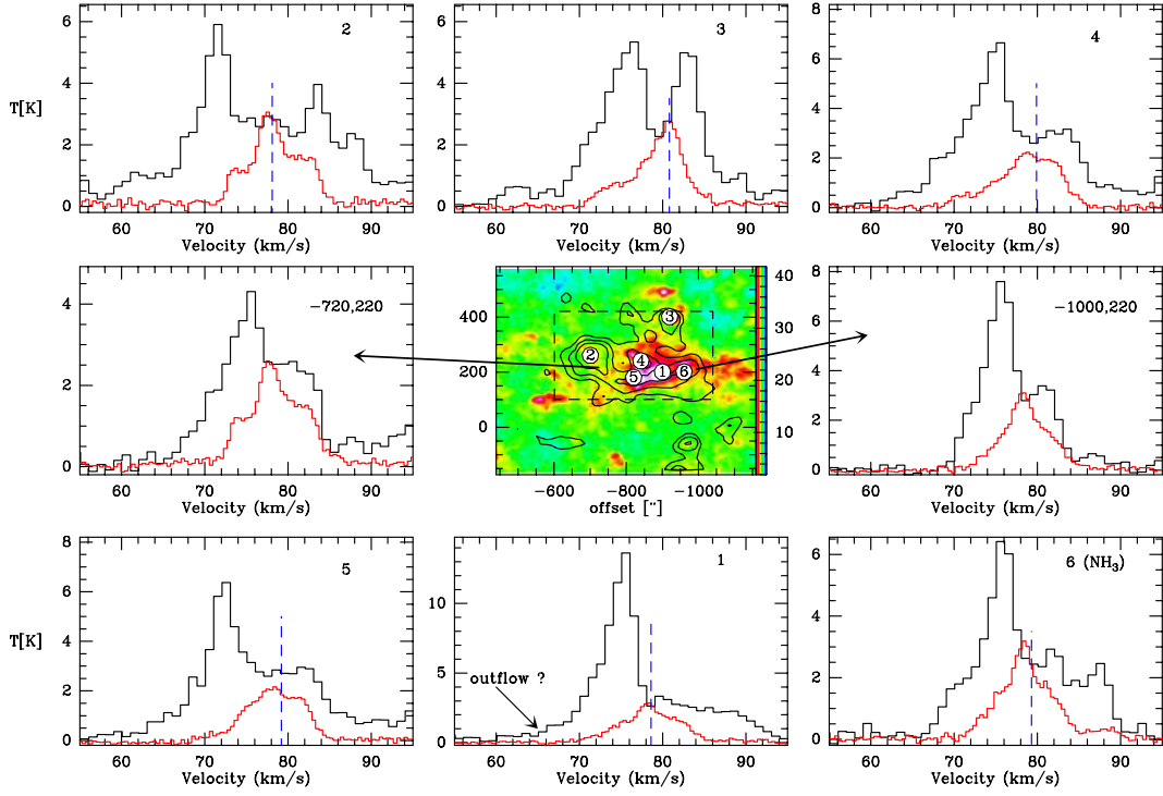
Fig. 8. Middle panel shows in colour the line integrated ^{12}\text{CO} 3 \rightarrow 2 emission in \text{K km s}^{-1} on a main beam temperature scale (between 72 and 84 \text{km s}^{-1} ) of G28.37+0.07. The dust column density from Herschel is overlaid as black contours (levels 4, 5, 7 10^{22} \text{ cm}^{-2} ). The dashed lines outline the area displayed in Fig. 9, and the numbering from 1 to 6 indicates the position of submm-continuum sources seen with ATLASGAL and subsequently observed in \text{N}_2\text{H}^+ (Tackenberg et al. 2014). The ^{12}\text{CO} 3 \rightarrow 2 (black) and ^{13}\text{CO} 1 \rightarrow 0 (red) spectra at these positions are displayed in the panels around. Additionally, we show spectra from two positions (indicated by arrows) off the sources but still within the molecular cloud. The blue-dashed line denotes the centre velocity of the \text{N}_2\text{H}^+ line.
