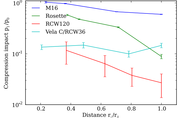
Fig. 12. Radial evolution of the ratio of the number of pixels in the compressed peak to the number of pixels in the low-density peak p_1/p_0 for the four different clouds.
