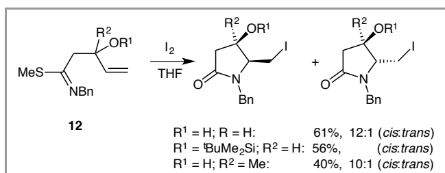
Scheme 9 Iodocyclization of unsaturated thioamidates.
