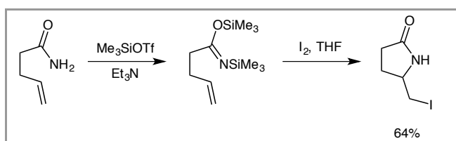
Scheme 8 Iodoaminocyclization of bissilylated iminoesters
