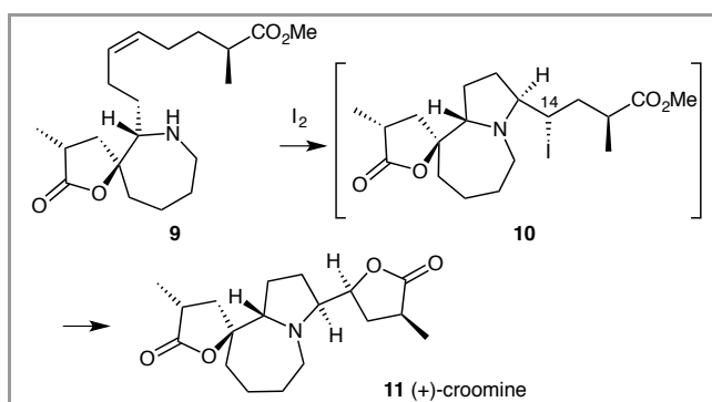
Scheme 6 Synthesis of (+)-croomine 11 .
