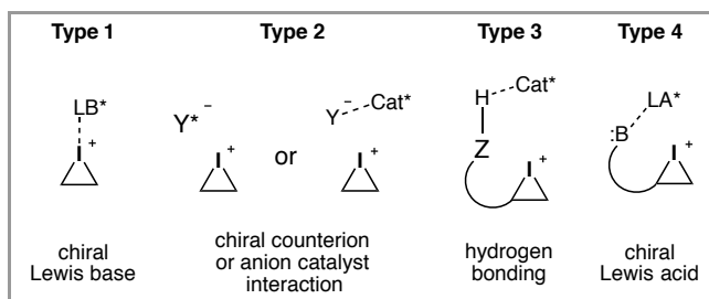
Figure 1 Strategies for stereoselective iodinations.
