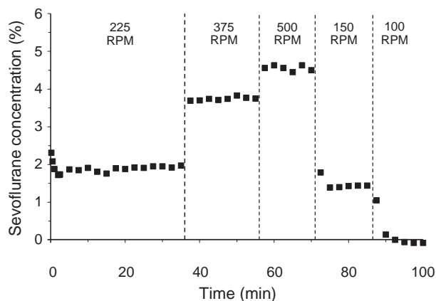
Figure 3 Sevoflurane output concentrations of the anaesthetic delivery device at various stirring rates with an input flow of 1 \text{ l} \cdot \text{min}^{-1} nitrogen at 20^\circ \text{C} .
