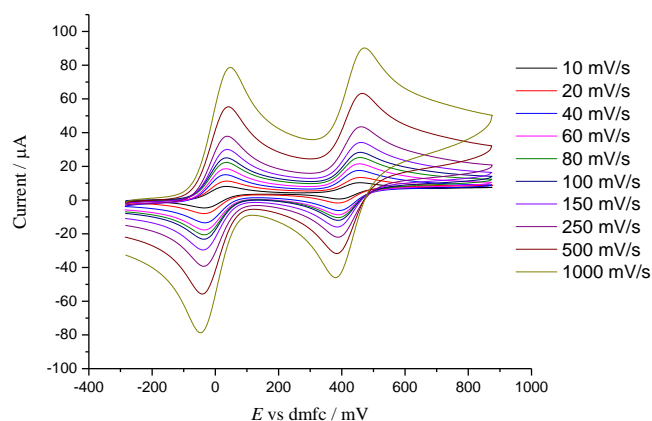
Figure 4. Cyclic voltammograms of 1 -( S,R p ) at various scan rates wrt decamethylferrocene. Concentration 1.0 mM with 0.1 M TBAPF 6 in dry acetonitrile at RT.
