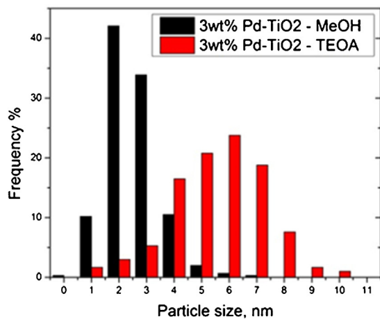
Fig. 2. TEM images of 3% Pd-C 3 N 4 after reaction with A) MeOH B) TEOA and 3% Pd-TiO 2 after reaction with C) TEOA and D) MeOH. The particle size histograms are also shown, obtained from counts of more than 300 nanoparticles.
