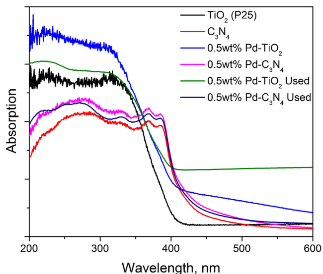
Fig. 1. UV-vis absorption spectra of pure TiO 2 (P-25) and C 3 N 4 , and with 0.5% Pd loaded, both before and after use.
