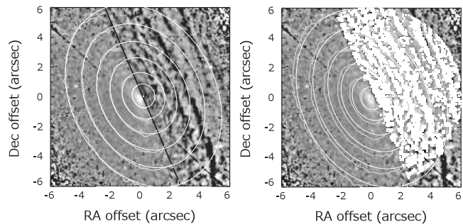
Figure 7. Left: Alternative MGE model (red contours) created by using data only on the left side of the green line. The contours are overlaid on an unsharp-masked HST H -band (NICMOS F160W) image (blue contours and grey scale). Right: Another MGE model (red contours) created by masking all the pixels indicated in green, overlaid to the unsharp-masked HST H -band (NICMOS F160W) image (blue contours and grey scale).
