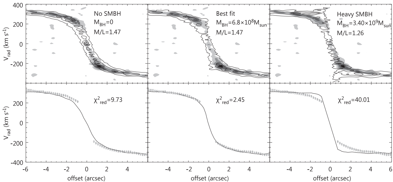
Figure 10. Upper panels: Observed position-velocity diagram (PVD) along the kinematic major axis (greyscale), overlaid with the model PVDs (contours). The left panel shows a comparison with a model without a black hole ( M_{\text{BH}} = 0 ), the middle panel with the best fit, and the right panel with an overweight black hole. Lower panels: Extracted mean velocities along the kinematic major axis (red points with error bars), overlaid with the best-fit model velocities (black lines). The reduced \chi^2 of each model is 9.73 (left, M_{\text{BH}} = 0 ), 2.45 (middle, best fit) and 40.01 (right, overweight SMBH).
