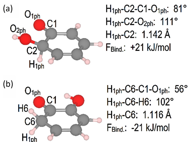
Fig. 15. Catechol-derived cyclo-hexadienones from the MOA with non-planar configuration. (a) cyclohexa-3,5-dien-2-hydroxy-1-one, derived from the H_{1ph} transfer to C2 that binds the second O_{2ph} ; (b) cyclohexa-2,4-dien-2-hydroxy-1-one, derived from the H_{1ph} transfer to C6. Hydrogen atoms are shown in white, C in dark grey and O in red. Relevant dihedral and bond angles, together with interatomic distances are shown. (For interpretation of the references to color in this figure legend, the reader is referred to the web version of this article.)
