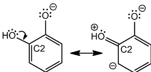
Scheme 3. Representation of resonance structures related to the \pi conjugation of the electronic lone pair of the second O_{2ph} atom with the aromatic ring.
