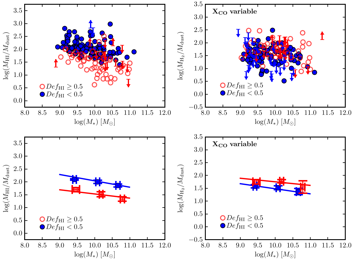
Figure 4. The M_{\text{HI}}/M_{\text{dust}}-M_* (left) and M_{\text{H}_2}/M_{\text{dust}}-M_* (right) relations for H I-normal (filled blue) and H I-deficient (empty red) HRS galaxies. Individual galaxies are shown in the upper panels, with circles and arrows indicating detections and upper/lower limits, respectively. Averages per bin of stellar mass and best linear fits are shown in the bottom panels.
