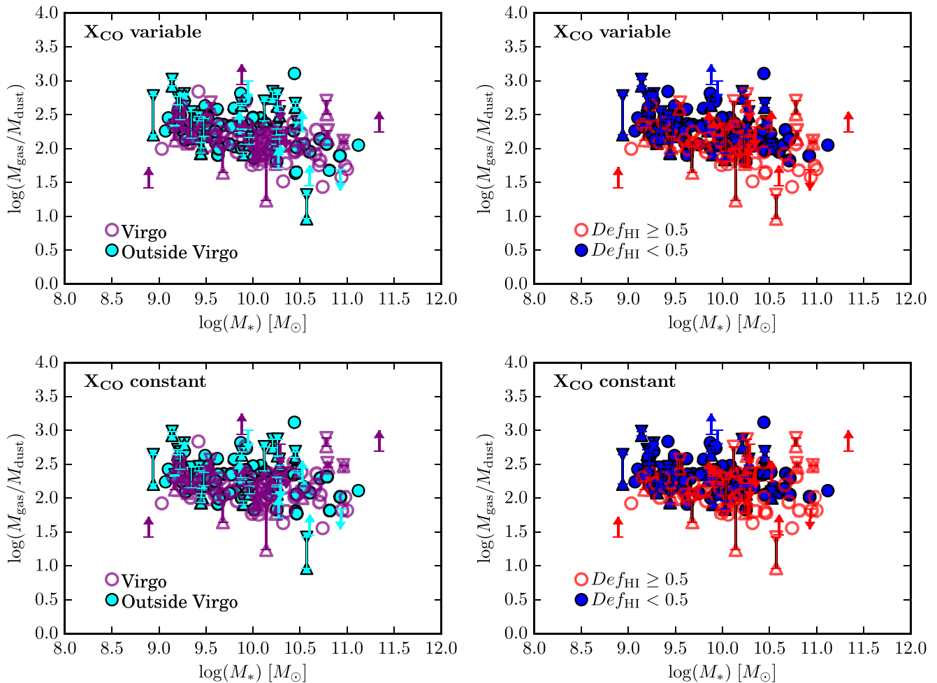
Figure 2. The M_{\text{gas}}/M_{\text{dust}}-M_* relation for galaxies in the HRS. Circles and arrows indicate detections and upper-limits, respectively. Interval censored data (i.e. galaxies for which dust and only one gas phase are detected) are presented as connected triangles, showing the possible range of variation in M_{\text{gas}}/M_{\text{dust}} obtained by setting the non-detected phase to either zero or its 5\sigma upper limit. The left column shows a comparison between Virgo cluster members (empty purple) and galaxies outside the Virgo cluster (filled cyan), whereas in the right column galaxies are divided according to their H I content, with H I-deficient and H I-normal galaxies as red empty and blue filled symbols, respectively. The top and bottom rows show results obtained for a variable and constant CO-to-H 2 ( X_{\text{CO}} ) conversion factor, respectively.
