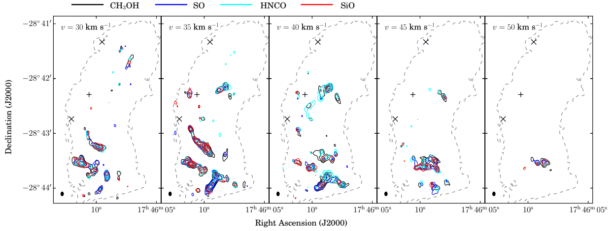
Fig. 8. SMA \text{CH}_3\text{OH} 4(2, 2)–3(1, 2)-E, SO, HNCO and SiO emission. Contours are -5, 5, 8, 12, 16 and 20\times the rms noise values for each line given in Table 1, for a spectral resolution of 5 \text{ km s}^{-1} . A synthesised beam of 4.3'' \times 2.9'' , \text{PA} = 0^\circ is shown in the bottom left corner. The plus sign marks the position of the water maser reported by Lis et al. (1994) and the crosses mark (from north to south, respectively) the positions of the 1.3 cm sources VLA 4 and 5 from Rodríguez & Zapata (2013). The dashed grey contour shows the combined dust continuum emission at a level of 0.024 \text{ mJy beam}^{-1} , the lowest solid black contour shown in Fig. 4.
