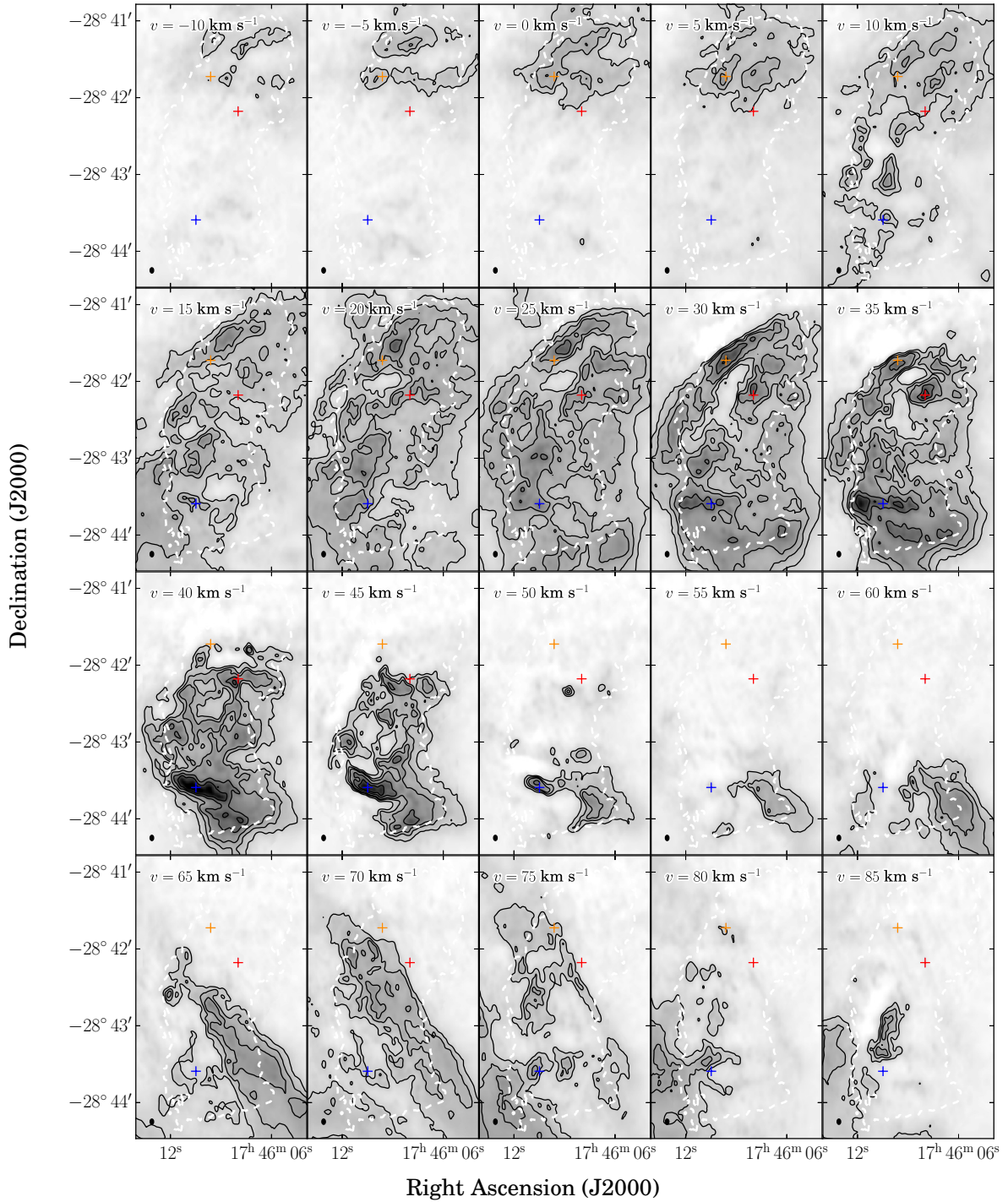
Fig. 11. Combined SMA + IRAM 30 m ^{13}\text{CO} emission between -10 and 85\text{ km s}^{-1} . Contours are 10, 15, 20, 30 and 40\times the map sensitivity 0.14\text{ mJy beam}^{-1} , for a spectral resolution of 5\text{ km s}^{-1} . The greyscale ranges from -0.14 to 8\text{ mJy beam}^{-1} . The beam size of 4.2'' \times 2.9'' , \text{PA} = 0.7^\circ is shown in the bottom left corner, which corresponds to the size of the SMA beam. The dashed white contour shows the combined 1.3\text{ mm} dust continuum emission at a level of 0.024\text{ mJy beam}^{-1} , the lowest black contour shown in Fig. 4. The coloured crosses correspond to the positions of the spectra shown in Fig. 12.
