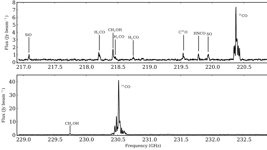
Fig. 7. Observed SMA spectra of both sidebands, averaged over the six observed fields for a short baseline (antennas 1 and 7).
