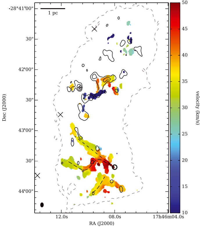
Fig. 9. First moment map of the 4(2,2)–3(1,2)-E methanol line at 218.440 GHz. Black contours show the 230.9 GHz or 1.30 mm continuum emission observed with the SMA at 5, 10 and 20 \times rms noise = 2.5 mJy beam ^{-1} . The synthesised beam for the methanol line is shown in the bottom left corner: 4.3'' \times 2.9'', PA = -1.1^\circ . The plus sign marks the position of the water maser reported by Lis et al. (1994) and the crosses mark (from north to south, respectively) the positions of the 1.3 cm sources VLA 4 to 6 from Rodríguez & Zapata (2013). The thick black circle in the south of the image marks the position of point A and the dashed lines show the positions of the three filaments mentioned in the text. The dashed grey contour shows the combined dust continuum emission at a level of 0.024 mJy beam ^{-1} , the lowest black contour shown in Fig. 4.
