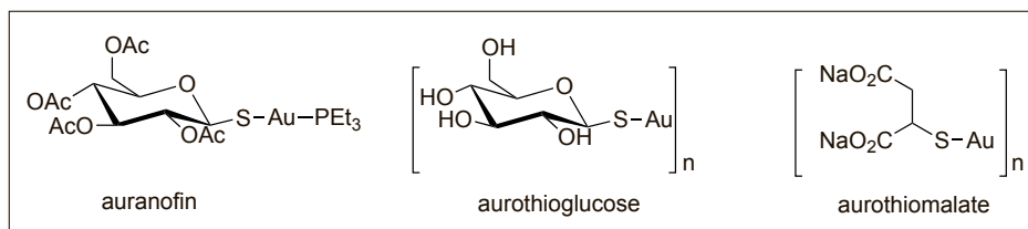
Fig. 1. Structures of Au(I) anti-rheumatic drugs.
