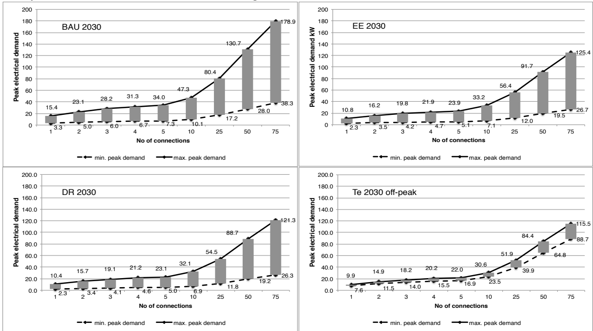
Figure 1: Winter peak demand range for gas heated communities in all scenarios
