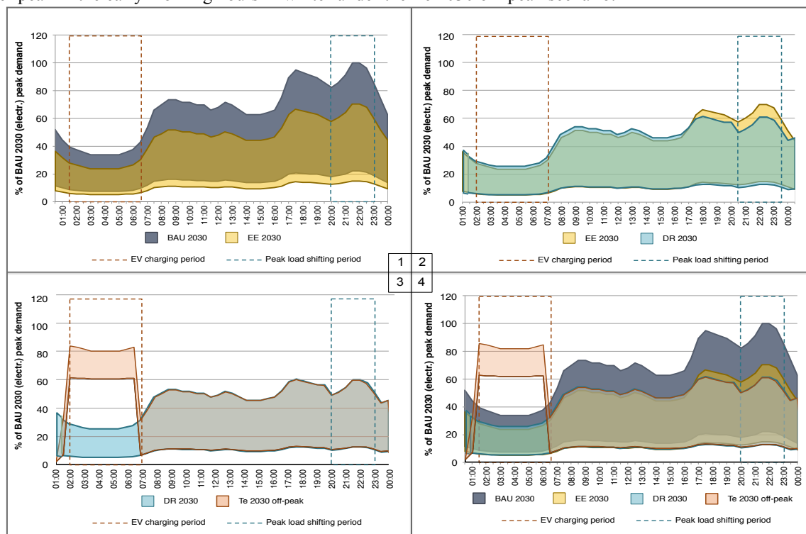
Figure 4: Evolution of load profiles in all scenarios for a single household on a summer weekday in 2030 (presented in ranges)
