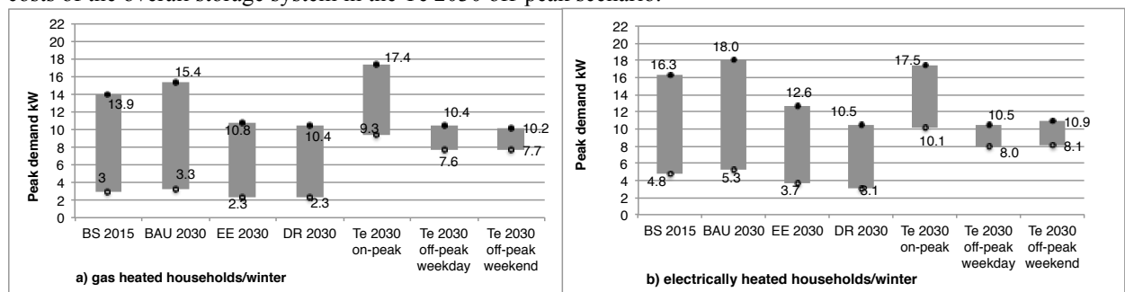
Figure 1: Winter electricity peak demand range for a) gas heated and b) electrically heated households in all scenarios
