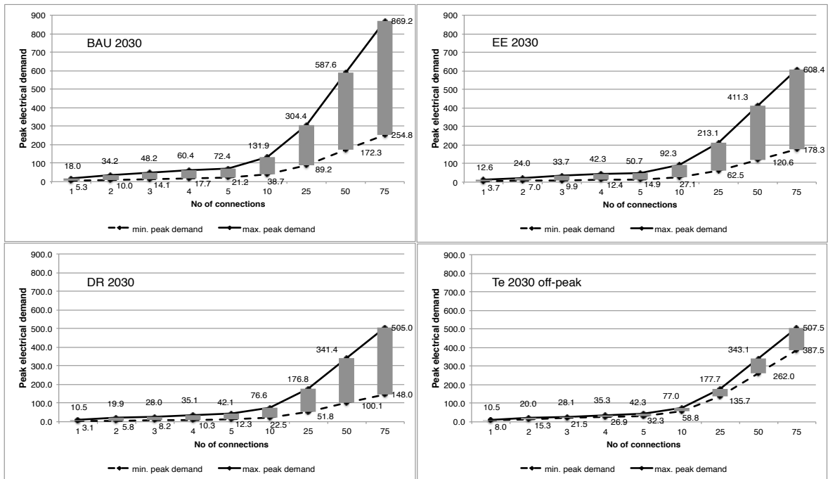
Figure 6: Winter peak demand range for electrically heated communities in all scenarios
