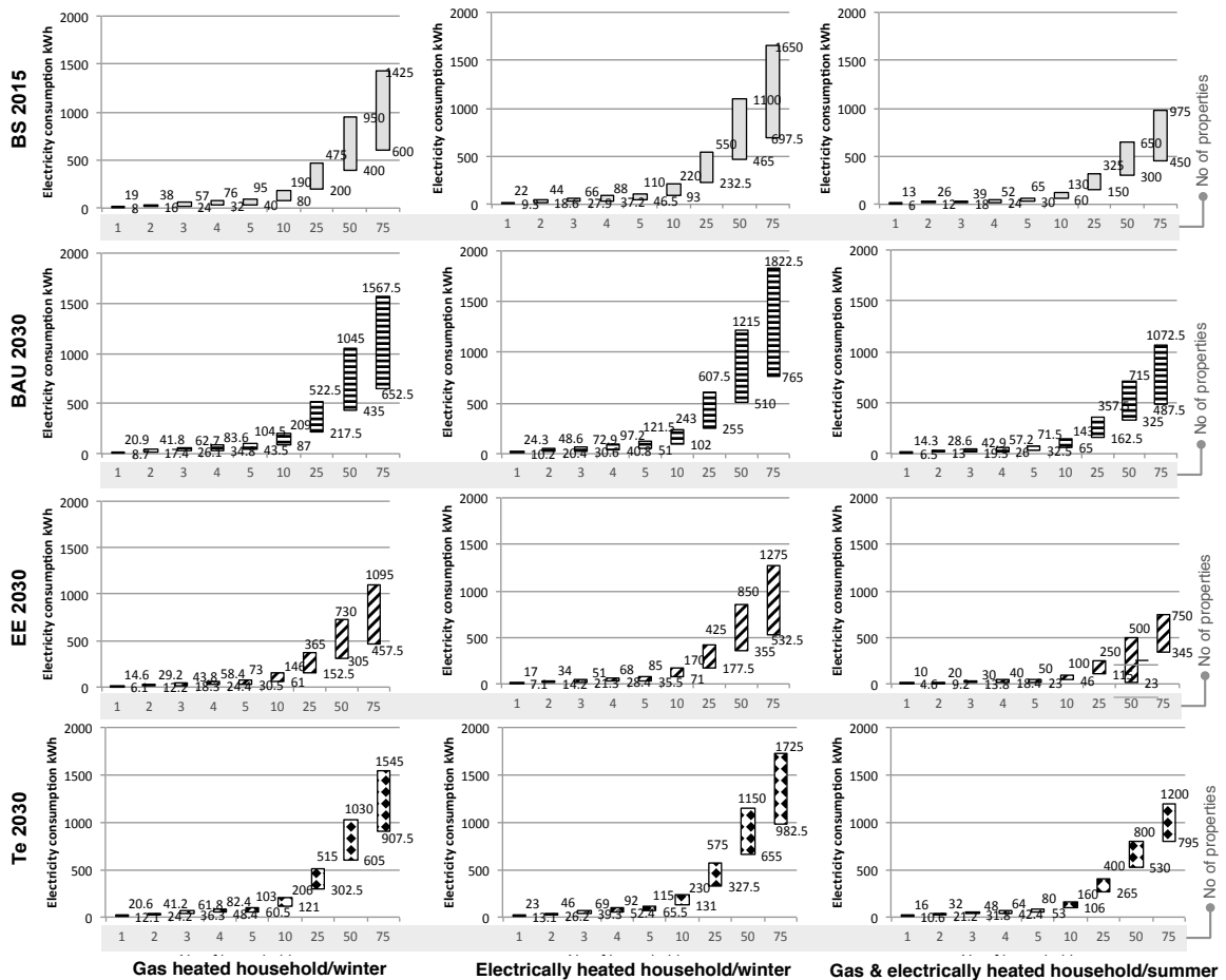
Figure 7: Electricity consumption range on weekends for different building scales in all scenarios
