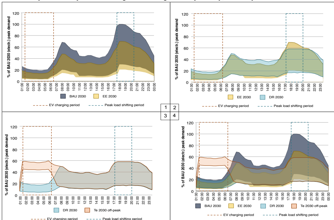
Figure 3: Evolution of load profiles in all scenarios for a single household on a winter weekday in 2030 (presented in ranges)
