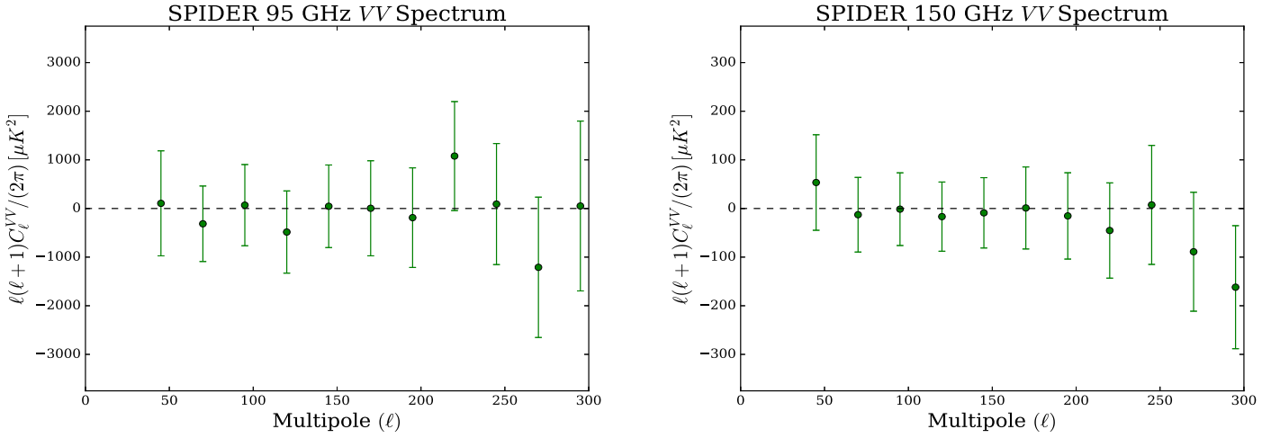
Figure 3. SPIDER’s VV angular power spectra at 95 and 150 GHz. The spectra are made by combining data on all three receivers at each frequency and include 68% C.L. error bars. The errors are obtained from Monte Carlo simulations based on the spread in the cross-spectra and the uncertainty in the circular polarization coupling of each HWP from Figure 1. The latter contribution is highly correlated across all \ell bins, leading to the visually low scatter in the points relative to the plotted errors. Note that the y-axis is a factor of 10 larger in the 95 GHz spectrum than in the 150 GHz spectrum.
