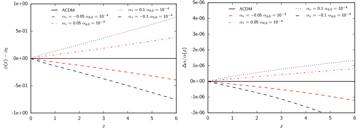
Figure 7: Field (left panel) and \Delta\alpha/\alpha (right panel) dependence on the \alpha_V parameter in the Dark Coupling case. While \phi(z) is anti-symmetric with respect to \alpha_V = 0 , the variation of \alpha preserves this symmetry only for small values of \alpha_V .
