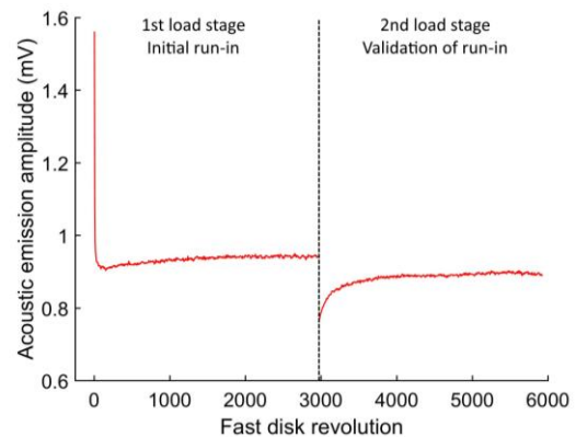
Figure 1. Initial running-in of disk set. Showing the mean Acoustic Emission band-passed between 150 - 300 kHz.
