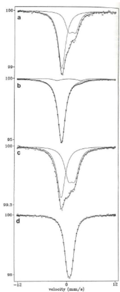
Fig. 4 ^{197}\text{Au} Mössbauer spectra of (a) 2% \text{HAuCl}_4/\text{C} absorbed on activated carbon from an aqua regia solution, (b) the same catalyst after deactivation at 180^\circ\text{C} for 6 h ( \text{GHSV} = 1140\text{ h}^{-1} , \text{C}_2\text{H}_2:\text{HCl} = 1:1.1 ), (c) a sample of the same type after reactivation by boiling in aqua regia, and (d) \text{HAuCl}_4 \cdot x\text{H}_2\text{O} . (Reproduced from Ref 49 with permission from Elsevier).
