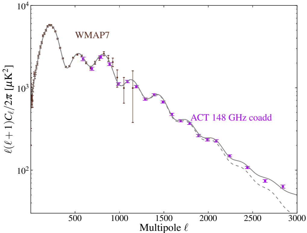
FIG. 1.— Data used in this cosmological analysis. The data from the WMAP 7-year data release (Larson et al. 2011; Komatsu et al. 2011) are combined with the ACT data. In this figure we show a weighted co-added spectrum from the equatorial and southern patches at 148 GHz. The full ACT likelihood, however, considers independent southern and equatorial spectra for both 148 GHz and 218 GHz (given in Table 3 of Das et al. 2013, and online on LAMBDA) and their cross-frequency spectrum, which are shown in Figure 2. The solid line indicates the best-fit cosmological model including foreground emission, while the dashed line shows the best-fit primordial CMB spectrum. This binning was selected for the common analysis of the equatorial and southern data. See Das et al. (2013) for alternative binnings.
