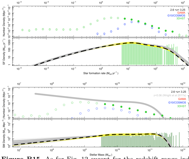
Figure B15. As for Fig. 12 except for the redshift range indicated.
