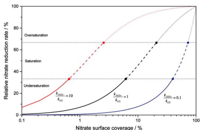
Fig. 2 The calculated relative nitrate reduction rate calculated according to eqn (23) assuming 50% relative humidity. The reaction constant for nitrate reduction is assumed to be identical (black) as well as ten times higher (red) or lower (blue) than the oxygen reduction constant, respectively. Also displayed is the expected regime for saturation if pure NO gas is used.
