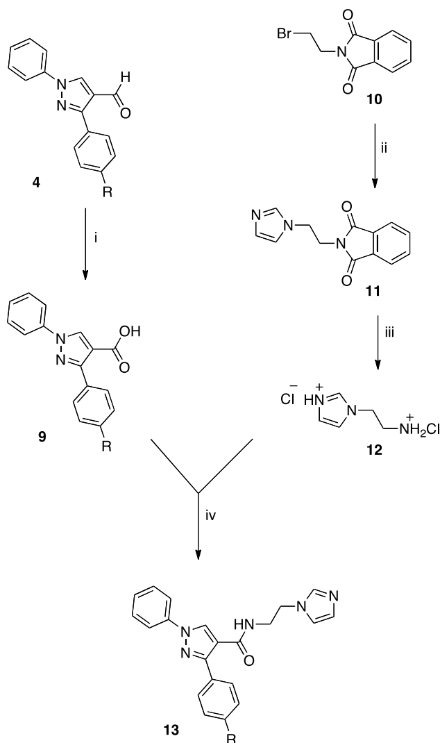
Scheme 2. Reagents and Conditions: (i) \text{KMnO}_4 , t\text{BuOH-H}_2\text{O} , 75\text{ }^\circ\text{C} , 45 min (ii) imidazole, 100\text{ }^\circ\text{C} , 3 h then toluene, 115\text{ }^\circ\text{C} , 20 h (iii) \text{NH}_2\text{NH}_2 , EtOH, reflux, 4 h (iv) CDI, DMF, 1 h then 12 , \text{Et}_3\text{N} , DMF, r.t., 20 h. [ a , R = H; b , R = 4-F; c , R = 4-Cl; d R = 4- \text{CH}_3 ; e , R = 4- \text{OCH}_3 ].
