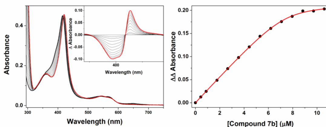
Figure 3. UV-Vis optical binding titration for compound 7b binding to CYP121A1. The left hand panel shows data from a compound 7b titration with CYP121A1 (~4.7 μM) with the ligand-free spectrum as a thick black line, spectra following progressive additions of 7b as thin solid lines, and the final near-saturated protein spectrum shown as a thick red line. The inset shows overlaid difference spectra generated by the subtraction of the starting spectrum from each consecutive ligand-bound spectrum collected in the titration. The right hand panel shows a plot of compound 7b -induced absorbance change – calculated as the difference between the peak and trough in the difference spectra in the left hand panel, using the same wavelength pair (429 and 392 nm, respectively) throughout. Data were fitted using the Hill equation to give a 7b K_D value of 4.16 \pm 0.47 μM.
