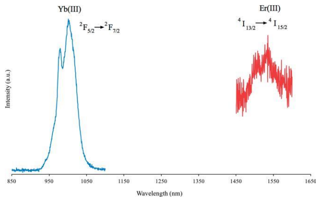
Figure 6. Near-IR solid-state emission spectra for \text{Er}^{3+} complex 7 and \text{Yb}^{3+} complex 9 .
