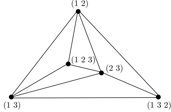
Figure 1: \overline{\mathcal{P}^*(S_3)} .
