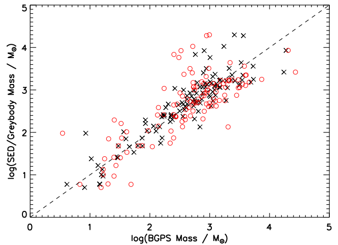
Figure 1. Comparison of SED-derived clump masses and masses calculated from the BGPS 1.1-mm flux density alone by Eden et al. (2013). The black crosses represent the BGPS masses calculated using the SED-derived temperature, whilst the red circles use a flat temperature of 14 K. The 1:1 line is indicated.
