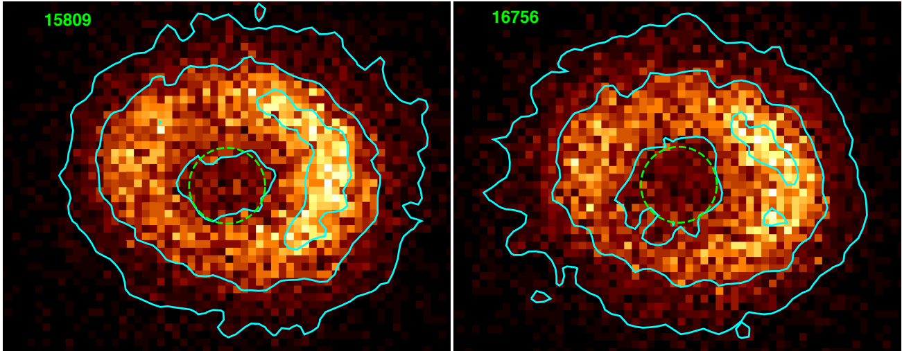
Figure 1. ACIS 2014 and 2015 images of SN 1987A in the 0.3–8 keV band with subpixel binning (1/8 of the native pixel size); the Obs.ID is indicated in each panel. The dashed circles show the area we considered to evaluate the limits (approximately 0''.3 radius). The brightest drawn contour levels in each panel correspond to \sim 25 counts \text{bin}^{-1} and the other levels are spaced by a factor of \sqrt{2} .
