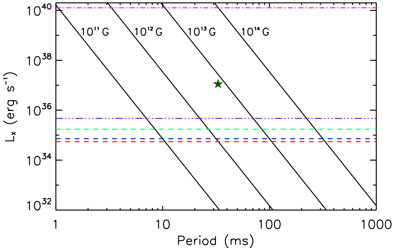
Figure 3. Constraints on the nonthermal emission from a neutron star. The solid black lines show the 2–8 keV X-ray luminosity as a function of the period for a few values of the magnetic field, as indicated by the labels. The dark green star marks the position of the Crab pulsar. The dashed lines indicate the 3\sigma upper limits obtained for different values of N_{\text{H}} : 3 \times 10^{21} (red), 3 \times 10^{22} (blue), and 1.8 \times 10^{23} \text{ cm}^{-2} (green). The three-dot-dashed line (violet) shows the extrapolation of the 2\sigma upper limit derived with INTEGRAL in the 20–60 keV band. The purple dot-dashed line indicates the limit derived for the absorption with abundances similar to those of the ejecta (see Section 2.2.3).
