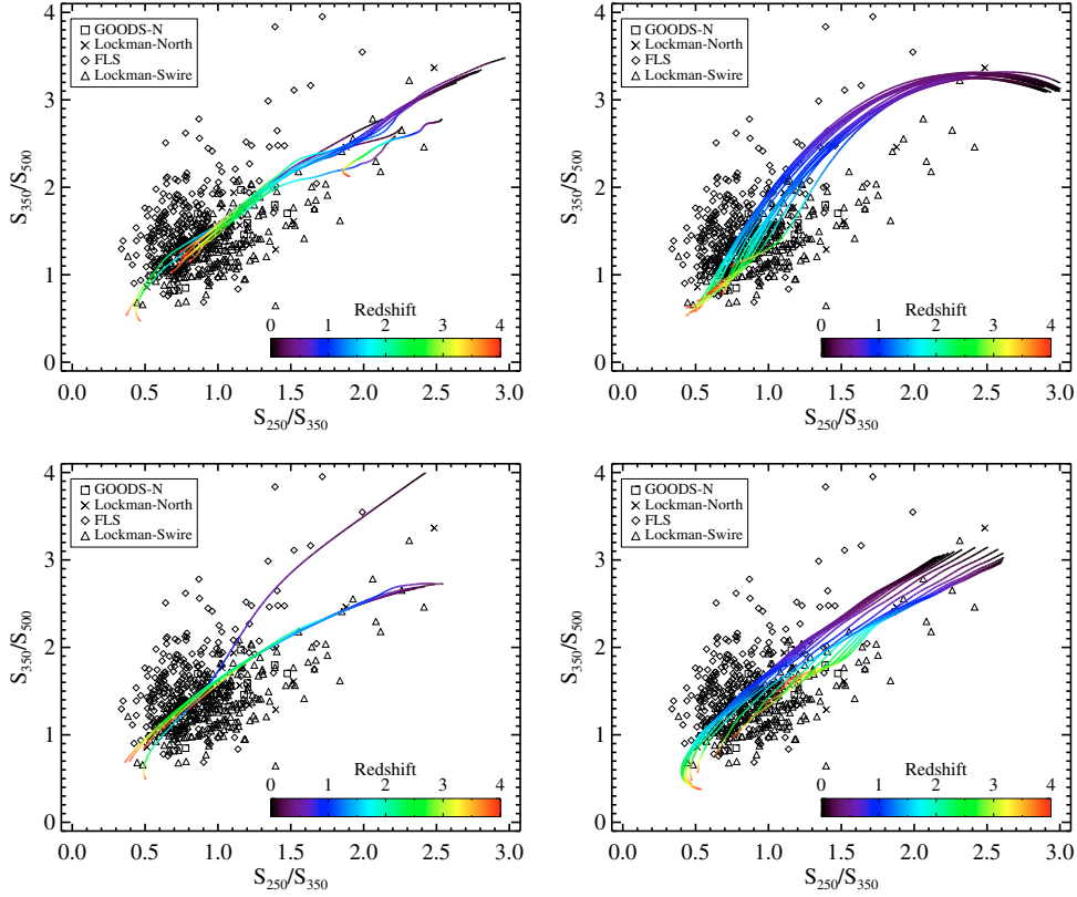
Fig. 3. S_{350}/S_{500} - S_{250}/S_{350} colour-colour plots for the SPIRE sources. Over plotted are the colour tracks from the galaxy evolution models of top-left Pearson et al. (2007), top-right Xu et al. (2001), bottom-left Lagache et al. (2003), and bottom-right Dale & Helou (2002). The redshift in the tracks is colour coded and runs from 0 to 4. The black symbols represent all unblended SPIRE sources according to the legend.
