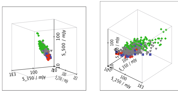
Fig. 2. The 3-dimensional flux parameter space for our unblended band-merged catalogues in the SPIRE 250, 350 and 500 \mu\text{m} bands. The sources in GOODS-N appear in red, Lockman-North in blue, FLS in grey, and Lockman-SWIRE in green. Both diagrams show the same 3D plot from two different aspect angles, the left one from within a plane fitted through the data, the other from a perpendicular direction.
