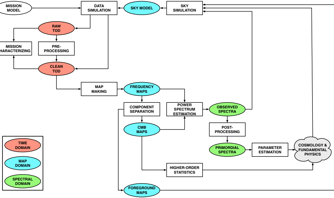
Figure 1. A schematic CMB simulation and analysis pipeline, with rectangular operators acting on oval data objects, which may be time samples (red), map pixels (blue) or spectral multipoles (green). Note the many loops, implying iterative processing.
