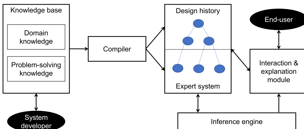
FIGURE 1 Explainable Expert System framework (adapted from Paris, 1993)
