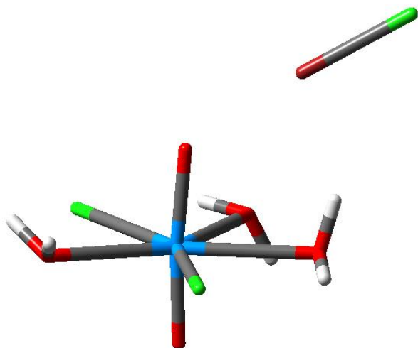
Figure 8: Optimised geometry of [\text{UO}_2\text{Cl}_2(\text{H}_2\text{O})_3]\dots\text{Br}-\text{Cl}
