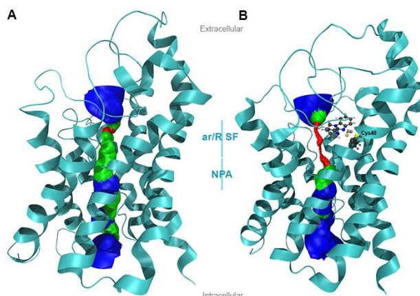
shown in ball and stick representation, with atoms coloured by atom type. Reproduced by permission of The Royal Society of Chemistry from 168 .
