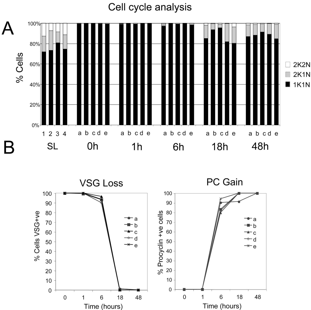
Figure 2 Cell cycle and surface antigen analysis during differentiation. A. Analysis of the percentage of cells in different cell-cycle phases (1 kinetoplast, 1 nucleus, Black; 2 kinetoplasts, 1 nucleus, grey; 2 kinetoplasts, 2 nuclei, white) from each of the bio-replicates and time points considered in this analysis. Most notably, the stumpy population is uniformly arrested in G1/G0 and cells progressing back into a proliferative cell-cycle begin to appear between 6-18 h after the initiation of differentiation. B. Expression of the bloodstream-stage specific variant surface glycoprotein (VSG) coat and EP procyclin (PC) coat on each of the bio-replicates and time points evaluated in this analysis. Samples were scored by immunofluorescence staining for the expression of each antigen. EP procyclin was weakly detectable at 1 h, but strongly expressed within 6 h.
