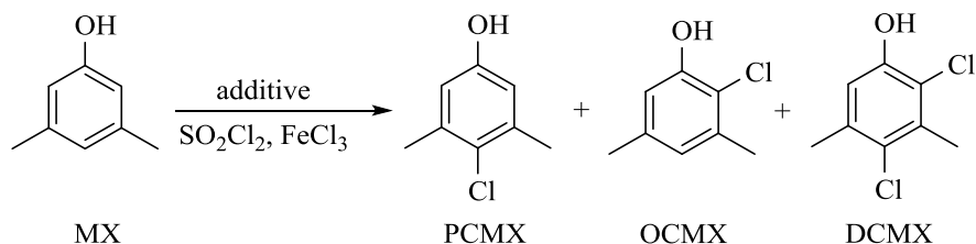
Scheme 1. Chlorination of m -xylenol.
