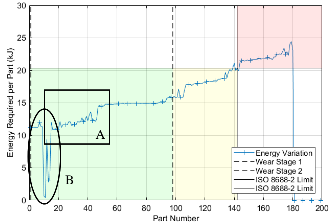
Figure 5. Estimated Stages of Tool Wear (SML)
