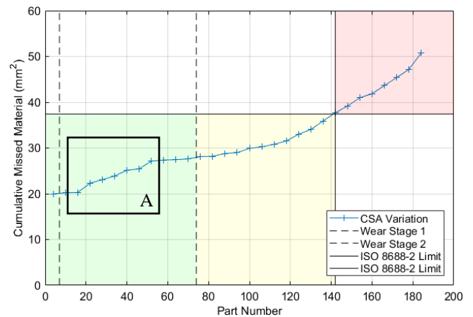
Figure 3. Estimated Stages of Tool Wear (GEO)
