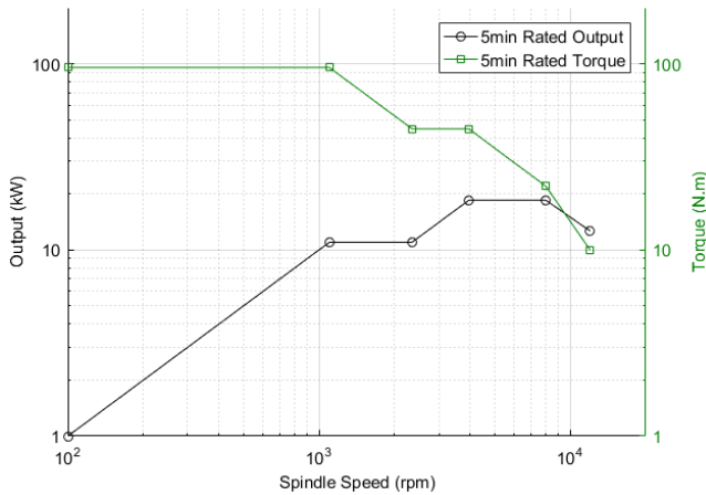
Figure 2. Spindle Motor Speed-Power-Torque Characteristic, Adapted from Mazak (2015)
