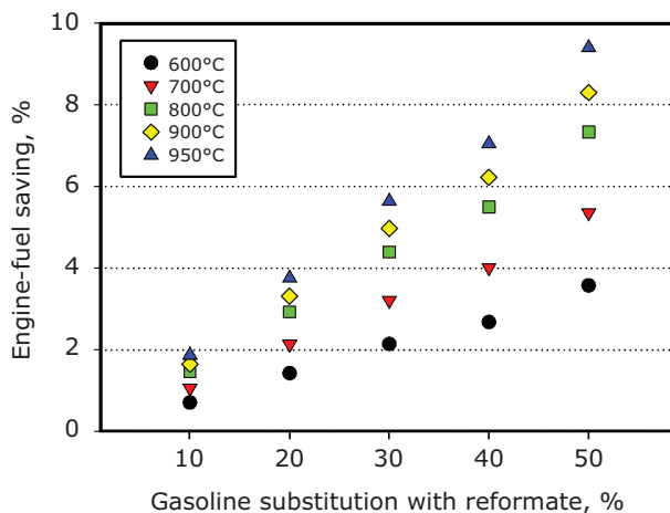
Fig. 10. Effect on predicted overall fuel savings achieved through fuel-by-reformat substitution in a gasoline engine, over a range of exhaust gas temperatures
