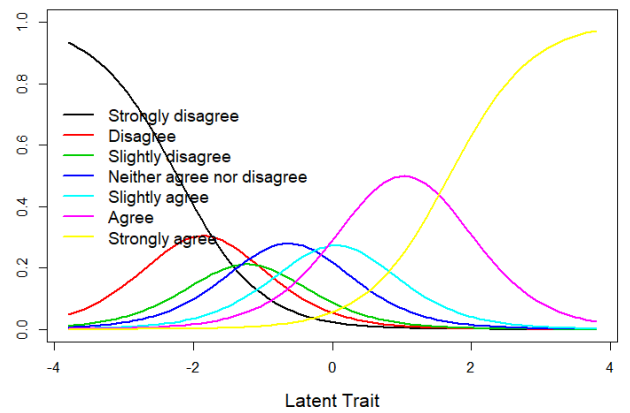
Item Response Category Characteristic Curves - Item: GCOS8
