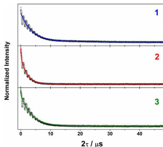
Figure 2. Comparison of the Hahn echo data (open circles) and corresponding biexponential fit (solid lines) for 1–3 recorded in 2% [\text{D}_7]\text{DMF}/\text{CD}_2\text{Cl}_2 at 10 K. Fit parameters are given in Tables S6–S8.
