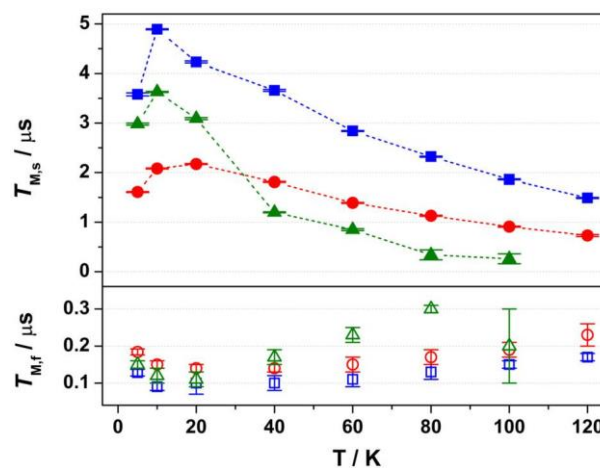
Figure 3. Comparison of the slow (top) and fast (bottom) contributions to phase memory time ( T_M ) for 1 (squares), 2 (circles) and 3 (triangles) over the temperature range 5–120 K. Error bars are based on the standard deviation of the fit (Tables S6–S8).
