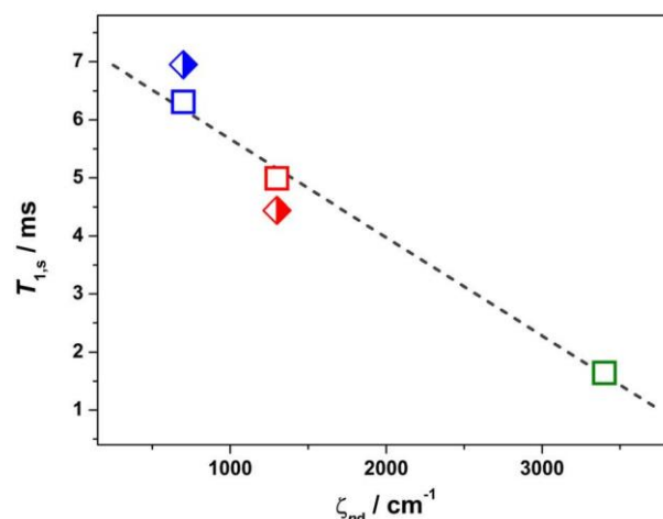
Figure 4. Linear correlation of the experimental spin-lattice relaxation time for 1 (blue), 2 (red) and 3 (green) on the spin-orbit coupling constant ( z ) for the metal ion. Diamonds represent the calculated T_{1,s} for 1 (blue) and 2 (red) relative to 3.
