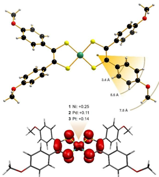
Figure 1. The molecular structure of [\text{Ni}(\text{adt})_2]^1 , showing distance of ligand protons from the spin barycenter (top), and the Mulliken spin density population from ZORA-PBE0 DFT calculations (bottom). The spin density at the metal ion in 1–3 is listed. Spin density is plotted with an isovalue 0.004 au.
