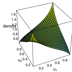
(e) Bel.Gre-Gaussian Copula
