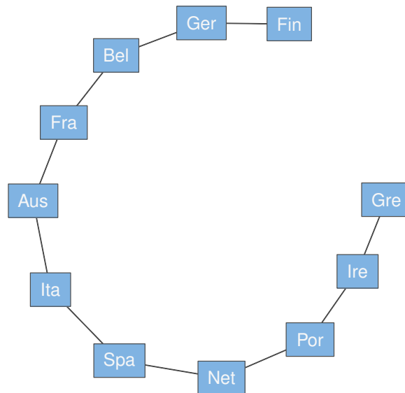
Figure 7: D-vine Tree level 1
